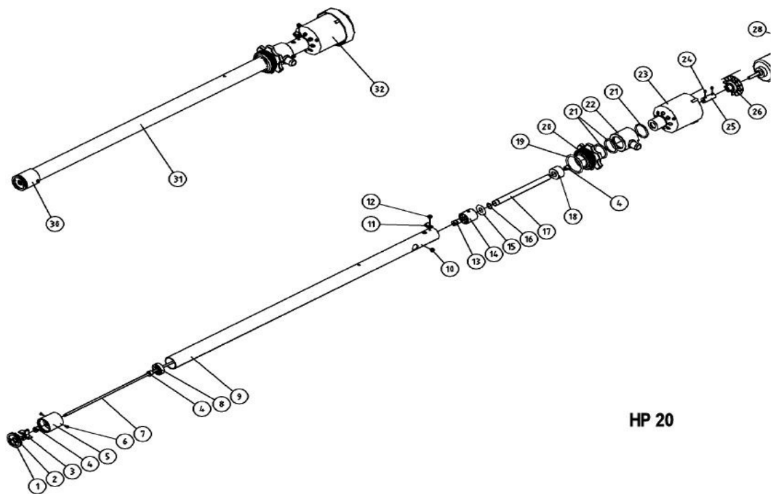
Partspicture No 11 Pump
