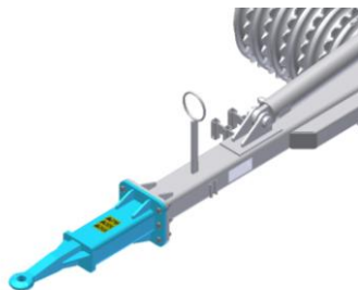
Hitch eye \varnothing 40mm
